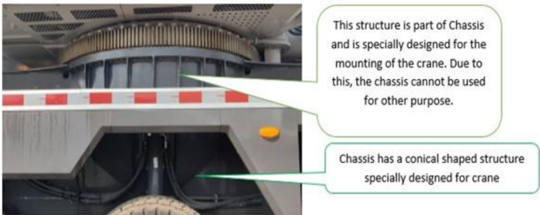
Pic-13 This picture shows the vehicle chassis specially designed for the crane
